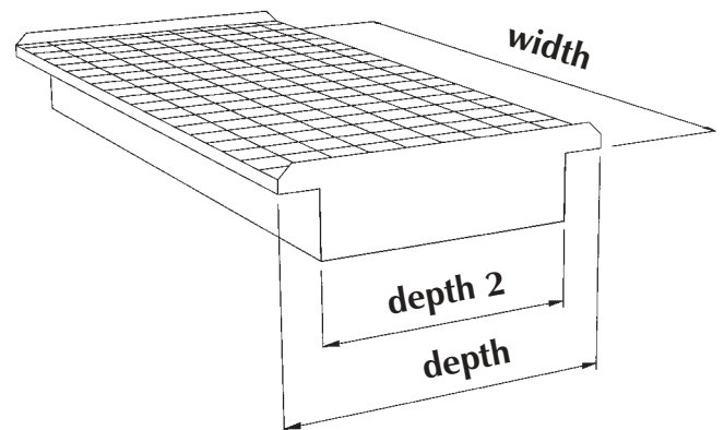
WSR-E 13.27/220, Article No. R23-5702-E, built into an existing pallet rack
