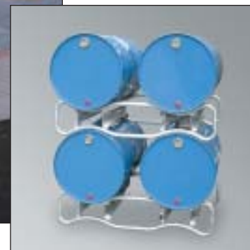
Drum pallet, filling height 230 mm, W x D x H mm = 1280 x 755 x 280, Article No. R67-1107-A
